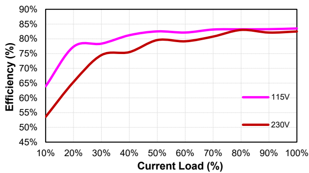
CFM40S090 (Eff Vs Io)
