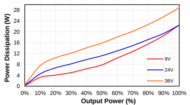
PS150W-24S28 Pd Vs Po @25 Deg. C
