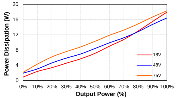
PS150W-48S24 Pd Vs Po @25 Deg. C
