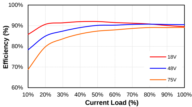
PS150W-48S28 Eff Vs Io @25 Deg. C
