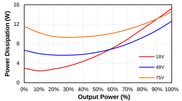
PS150W-48S05 Pd Vs Po @25 Deg. C
