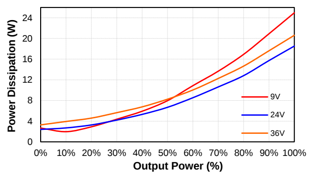
PS150W-24S15 Pd Vs Po @25 Deg. C
