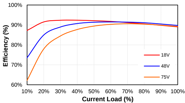
PS150W-48S12 Eff Vs Io @25 Deg. C
