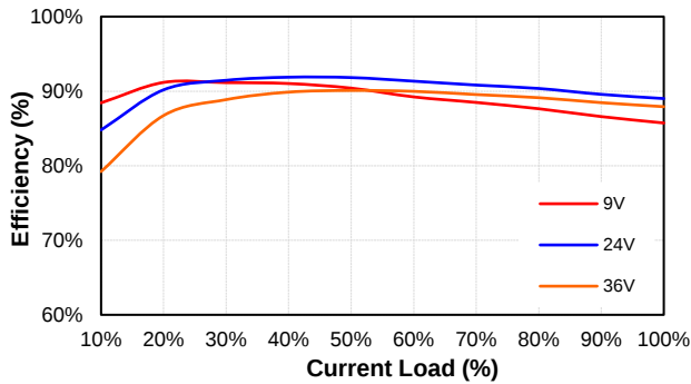
PS150W-24S15 Eff Vs Io @25 Deg. C
