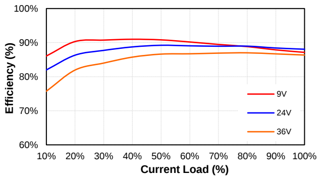
PS150W-24S28 Eff Vs Io @25 Deg. C
