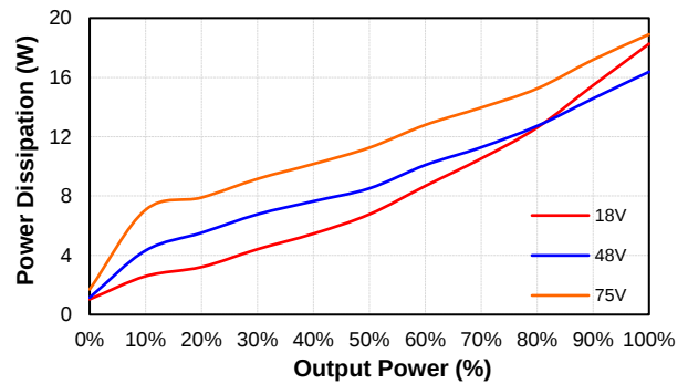
PS150W-48S28 Pd Vs Po @25 Deg. C
