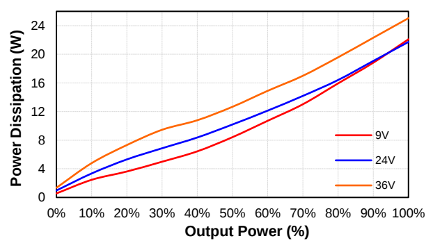
PS150W-24S24 Pd Vs Po @25 Deg. C
