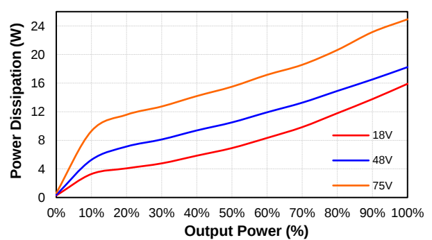
PS150W-48S48 Pd Vs Po @25 Deg. C
