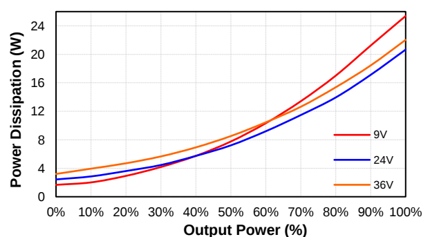
PS150W-24S05 Pd Vs Po @25 Deg. C
