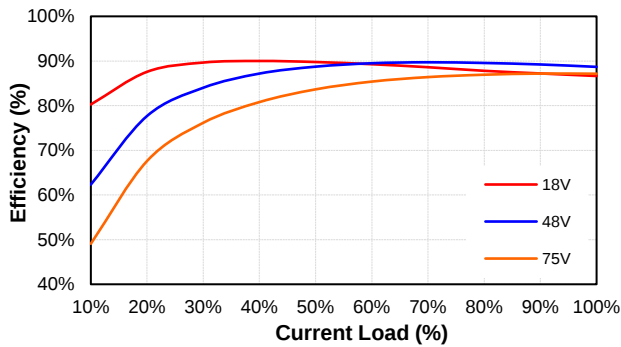
PS150W-48S05 Eff Vs Io @25 Deg. C
