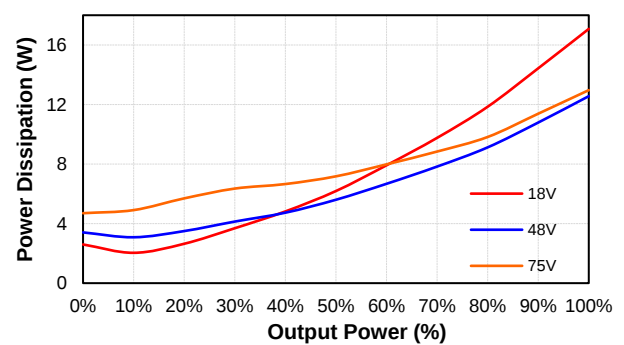
PS150W-48S12 Pd Vs Po @25 Deg. C
