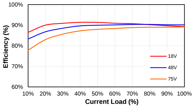
PS150W-48S24 Eff Vs Io @25 Deg. C
