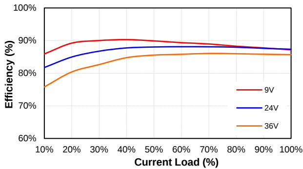
PS150W-24S24 Eff Vs Io @25 Deg. C
