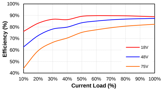
PS150W-48S48 Eff Vs Io @25 Deg. C
