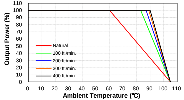
PS150W-48S12 Derating Curve with Heatsink HBT-254 (Vin=Nominal)
