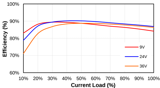
PS150W-24S05 Eff Vs Io @25 Deg. C
