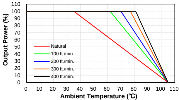
PS150W-48S12 Derating Curve with Heatsink HBT127 (Vin=Nominal)
