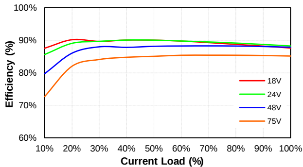
PS200W-48S24 Eff Vs Io @25 Deg. C
