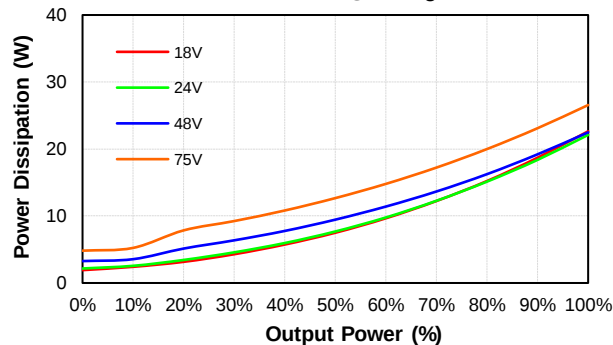
PS200W-48S05 Pd Vs Po @25 Deg. C
