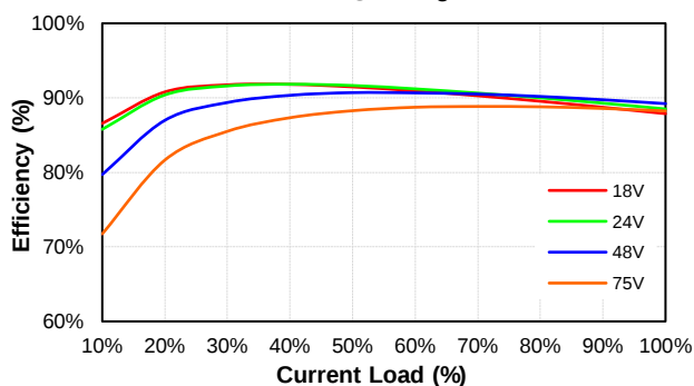
PS200W-48S3V3 Eff Vs Io @25 Deg. C
