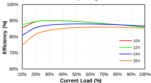
PS200W-24S15 Eff Vs Io @25 Deg. C
