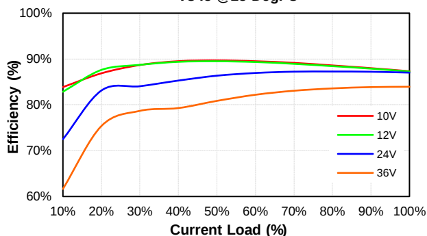
PS200W-24S48 Eff Vs Io @25 Deg. C
