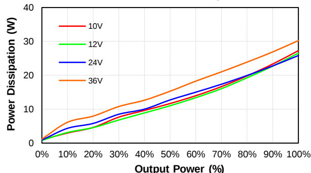
PS200W-24S28 Pd Vs Po @25 Deg. C
