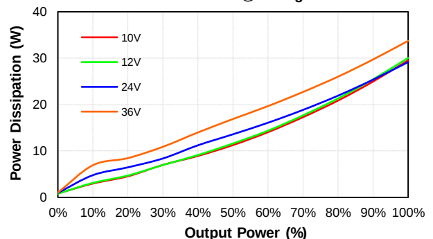
PS200W-24S24 Pd Vs Po @25 Deg. C
