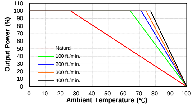
PS200W-48S05 Derating Curve with Heatsink HBT254
