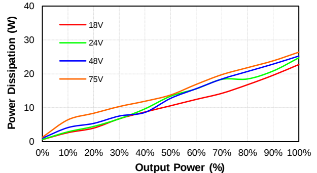
PS200W-48S28 Pd Vs Po @25 Deg. C
