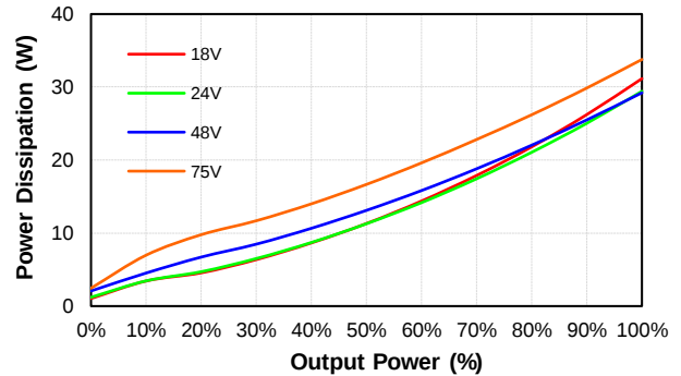
PS200W-48S12 Pd Vs Po @25 Deg. C
