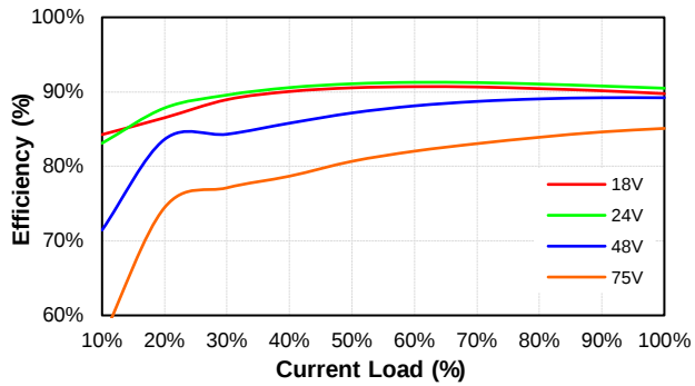
PS200W-48S48 Eff Vs Io @25 Deg. C
