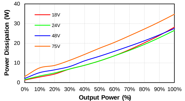
PS200W-48S24 Pd Vs Po @25 Deg. C
