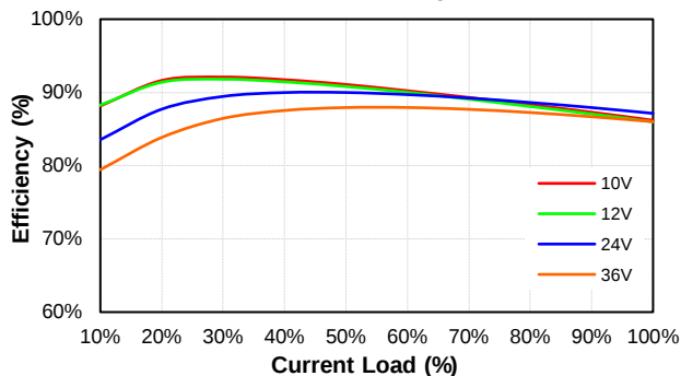
PS200W-24S05 Eff Vs Io @25 Deg. C
