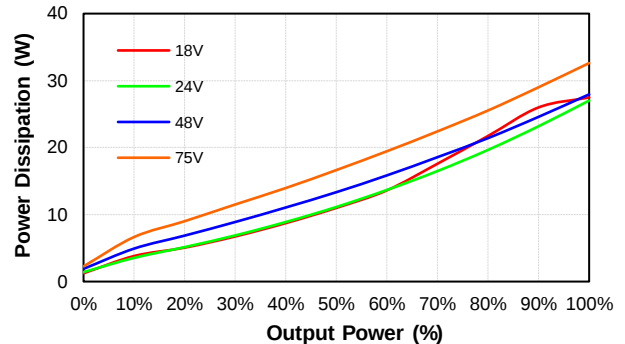
PS200W-48S15 Pd Vs Po @25 Deg. C
