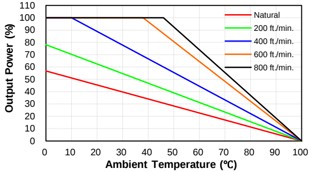
PS200W-48S05 Derating Curve without Heatsink
