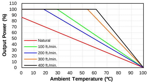
PS200W-48S05 Derating Curve with Heatsink HBT127
