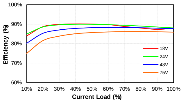
PS200W-48S15 Eff Vs Io @25 Deg. C
