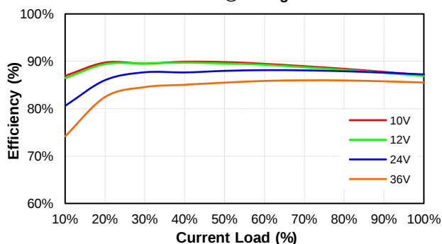
PS200W-24S24 Eff Vs Io @25 Deg. C
