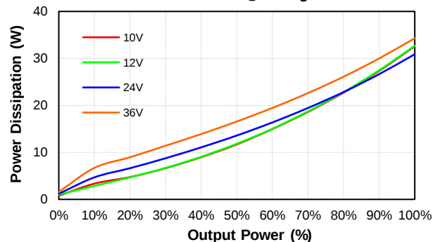
PS200W-24S15 Pd Vs Po @25 Deg. C
