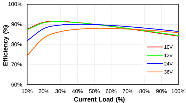
PS200W-24S3V3 Eff Vs Io @25 Deg. C
