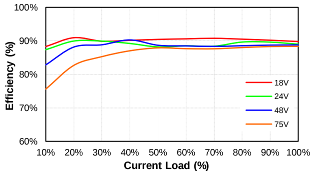
PS200W-48S28 Eff Vs Io @25 Deg. C
