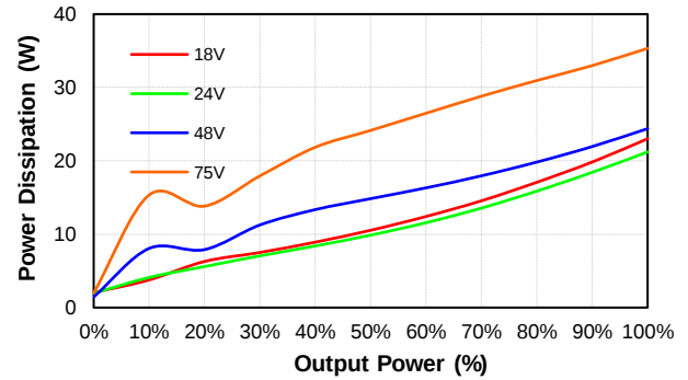
PS200W-48S48 Pd Vs Po @25 Deg. C
