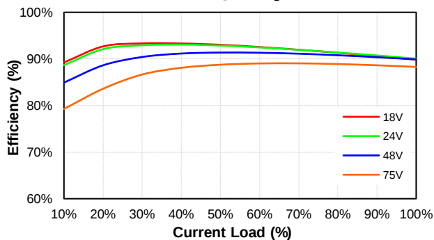
PS200W-48S05 Eff Vs Io @25 Deg. C
