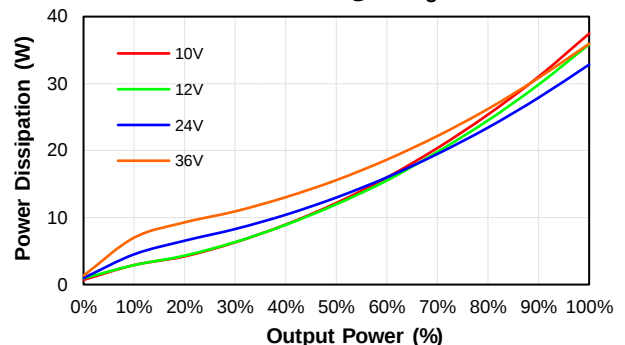
PS200W-24S12 Pd Vs Po @25 Deg. C
