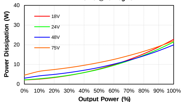
PS200W-48S3V3 Pd Vs Po @25 Deg. C
