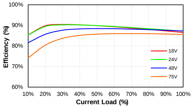
PS200W-48S12 Eff Vs Io @25 Deg. C
