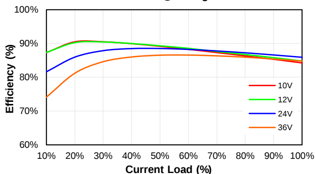
PS200W-24S12 Eff Vs Io @25 Deg. C
