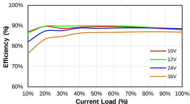
PS200W-24S28 Eff Vs Io @25 Deg. C
