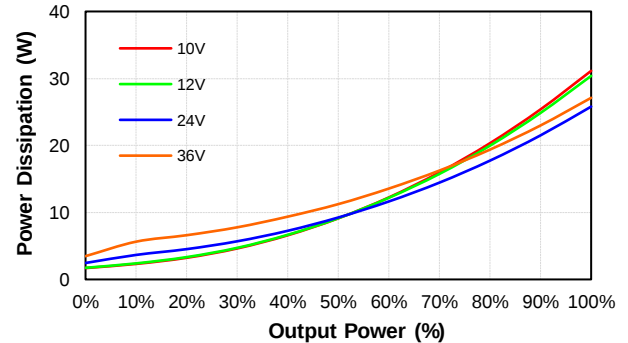
PS200W-24S3V3 Pd Vs Po @25 Deg. C
