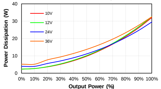
PS200W-24S05 Pd Vs Po @25 Deg. C
