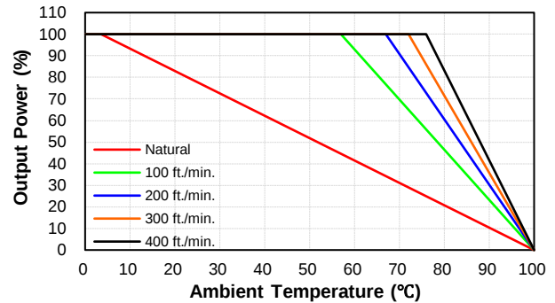
PS200W-48S05 Derating Curve with Heatsink HBL210
