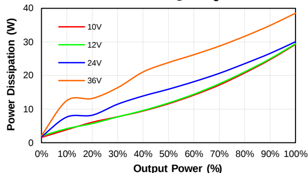
PS200W-24S48 Pd Vs Po @25 Deg. C
