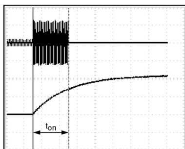
(Fig.5 limiting time T_{on} )
