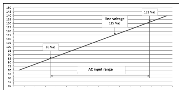
(Fig.4 operating range 115Vac)
