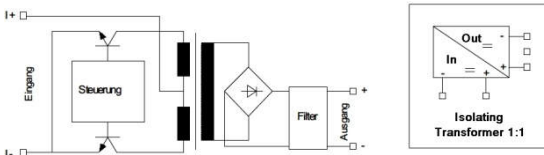
ADTW201 Isolating Transformer (fig5)
