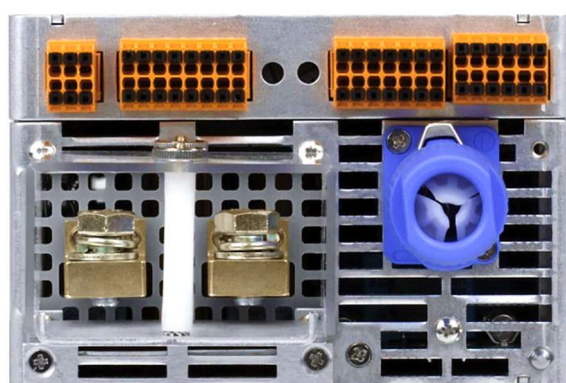
ANALOGUE INTERFACE
