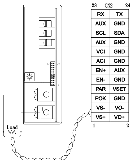
1. Remote Sense
