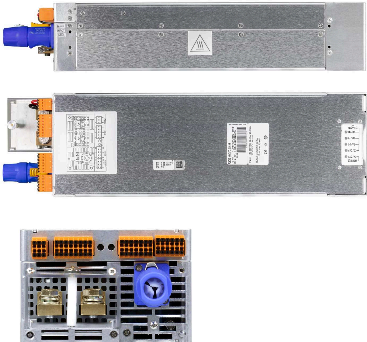
ANALOGUE INTERFACE
