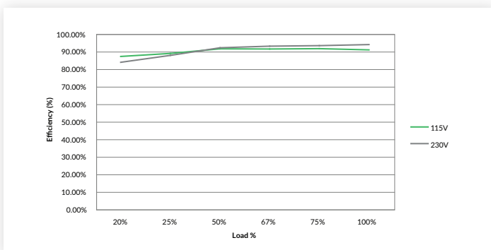
Figure 5 GCS150PS48
