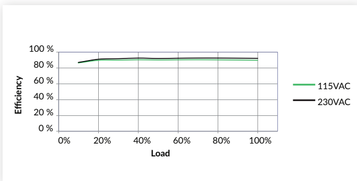
Figure 5 GSP500PS48
