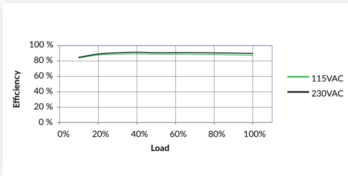
Figure 3 GSP500PS12
