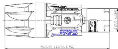
Neutrik NAC3FXXA-W-S
