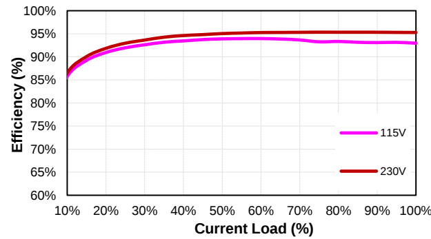
CBM300S280 (Eff Vs Io)
