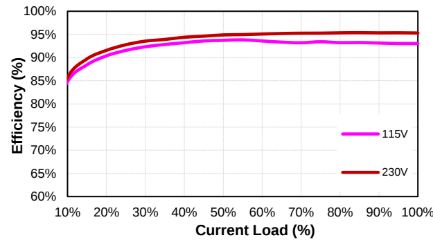
CBM300S480 (Eff Vs Io)
