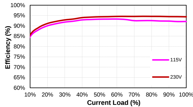
CBM300S150 (Eff Vs Io)
