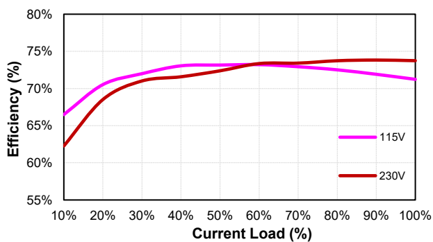
CFM40T-07 (Eff Vs Io)
