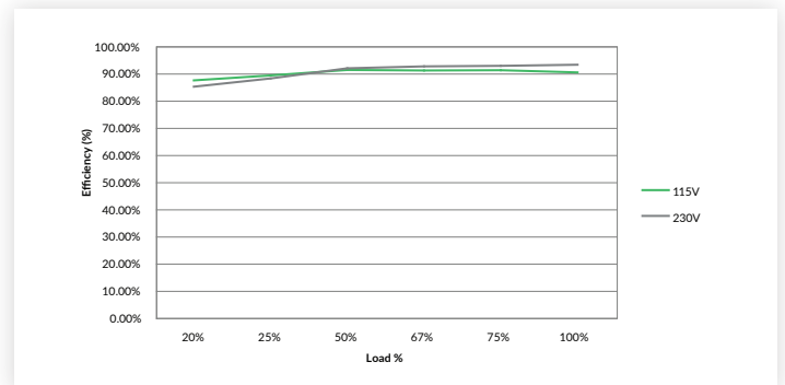
Figure 4 GCS265PS24
