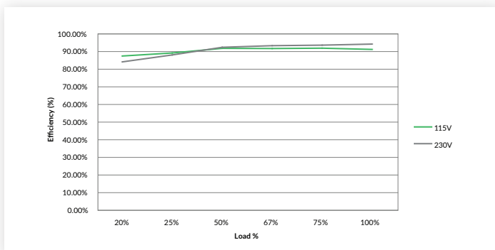
Figure 5 GCS265PS48
