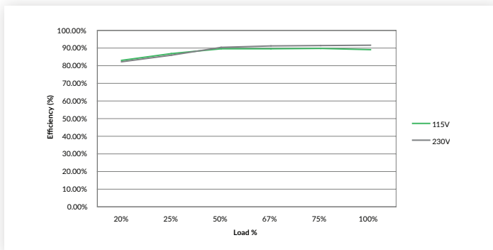
Figure 3 GCS265PS12
