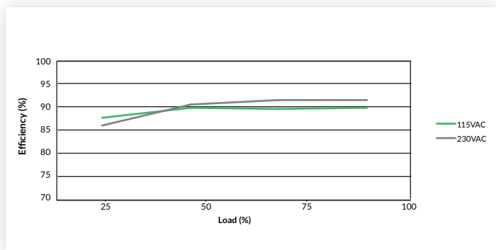
Figure 4 SMP350PS48
