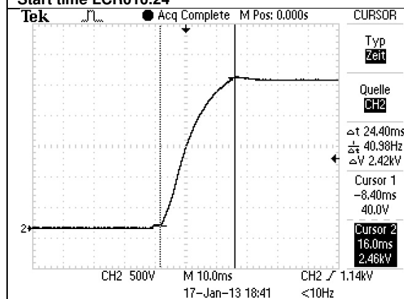
Start time LCR060.24
