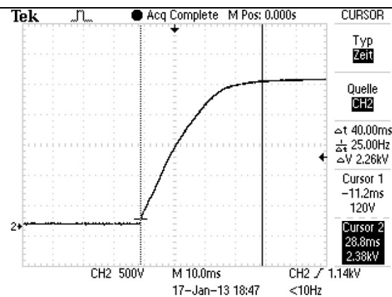
Start time LCR030.24
