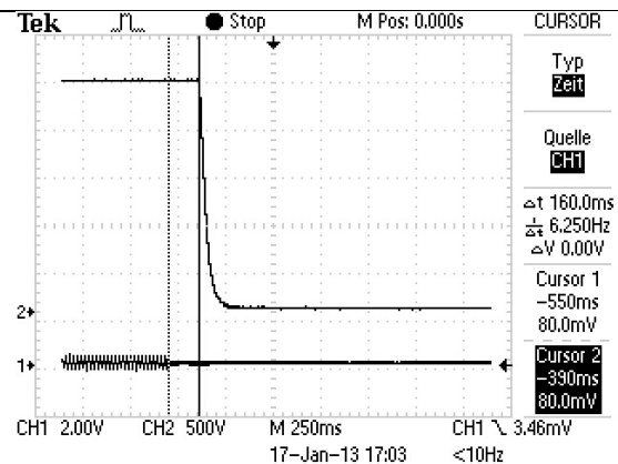
Hold-up time LCR030.24
