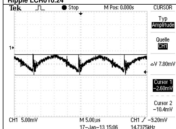
Ripple LCR060.24
