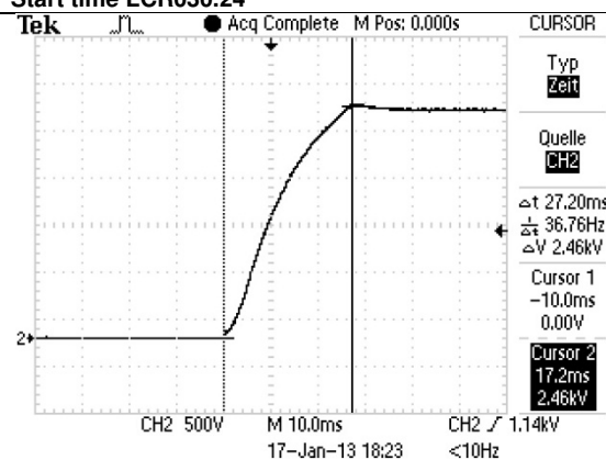
Start time LCR100.24
