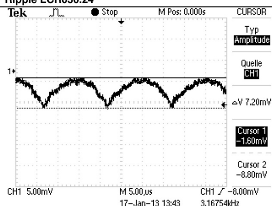
Ripple LCR100.24
