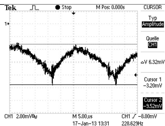
Ripple LCR030.24
