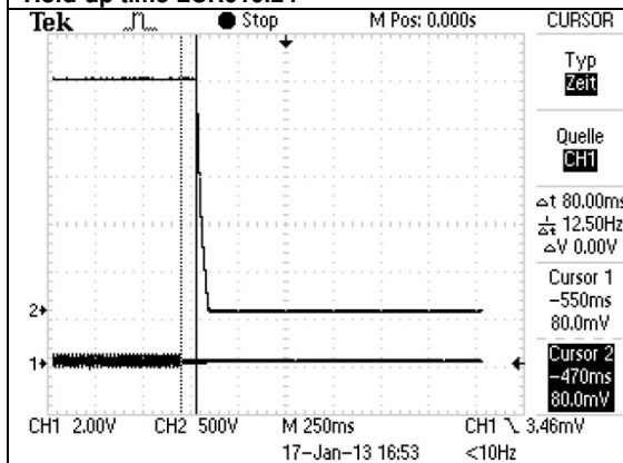
Hold-up time LCR060.24
