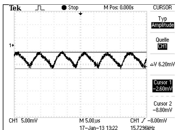
Ripple LCR010.24
