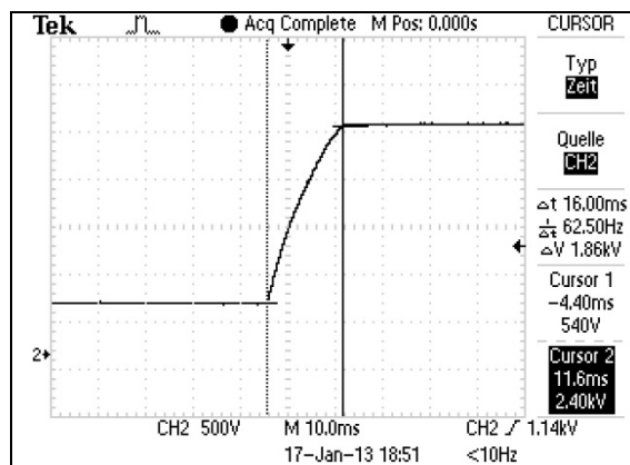
Start time LCR010.24
