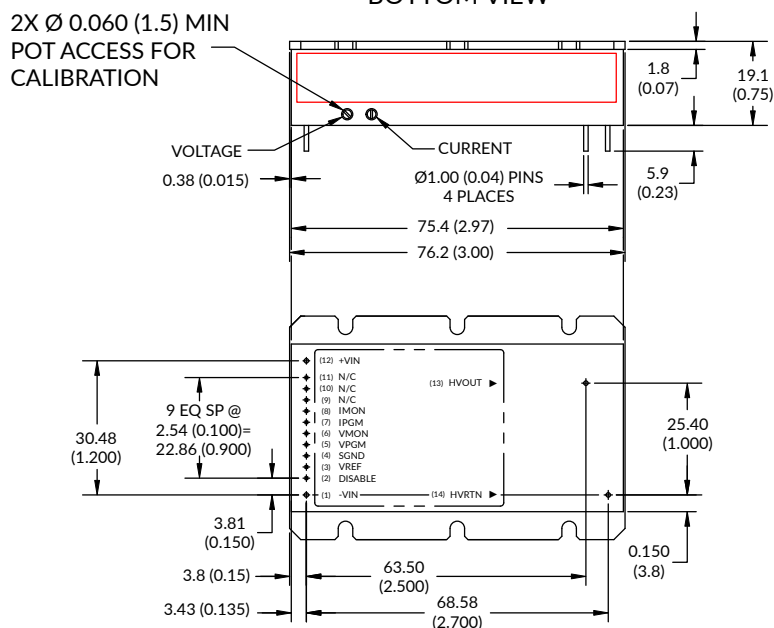
BOTTOM VIEW
