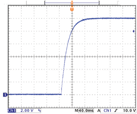
Figure 3 - V1 Typical no overshoot at start up.
