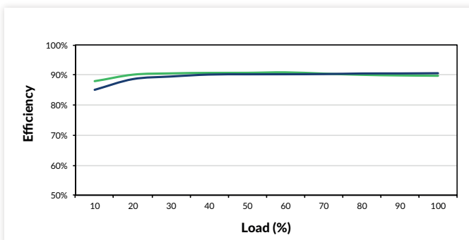
Figure 3 AEK40US24
