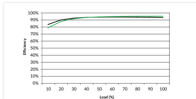
Figure 10 AHM250PS48
