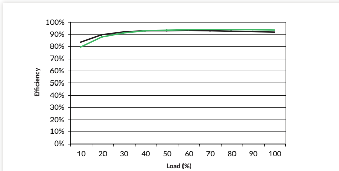
Figure 9 AHM250PS24
