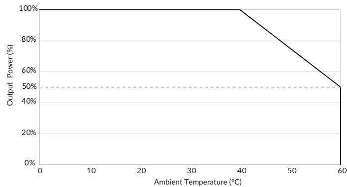
Ambient derating
