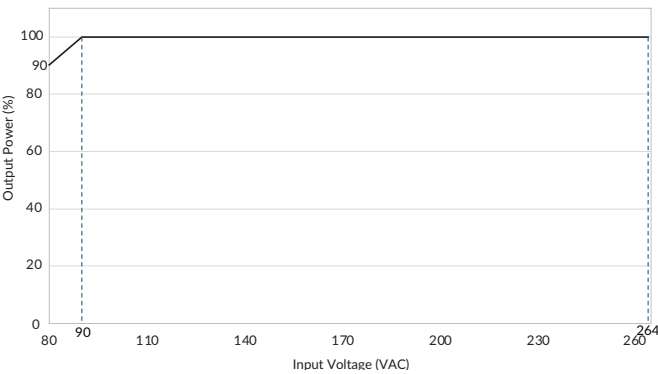
Input derating
