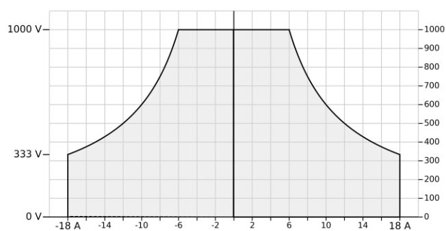
SM1000-CP-18
