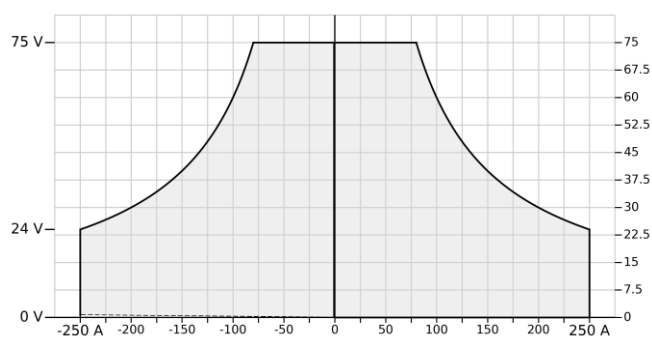
SM75-CP-250
